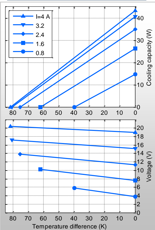
Performance Graphs at T_h=50^\circ\text{C}
