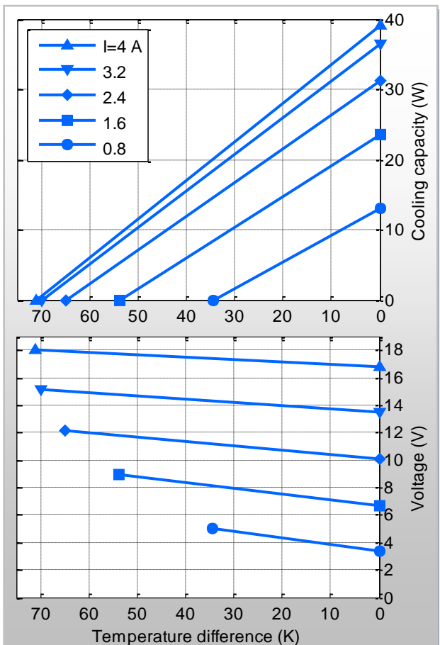
Performance Graphs at T_h=25^\circ\text{C}
