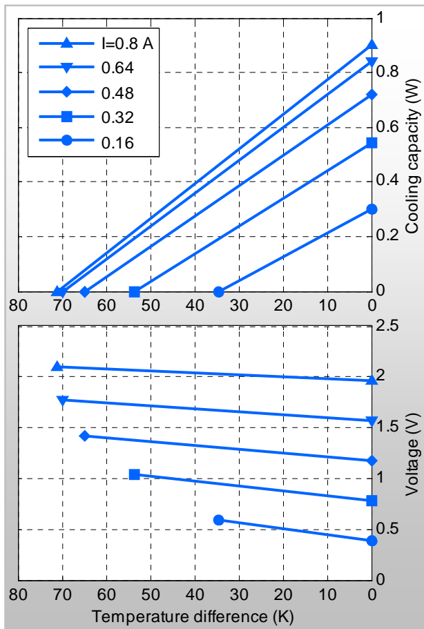
Performance Graphs at Th=25°C
