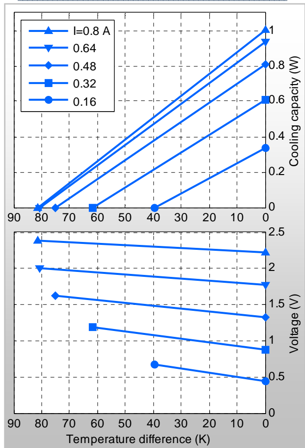
Performance Graphs at Th=50°C
