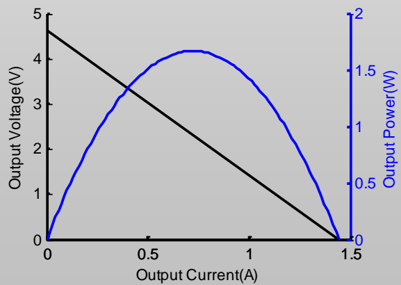
The chart for output voltage and output power Vs output current under Th=150 °C and Tc=50 °C
