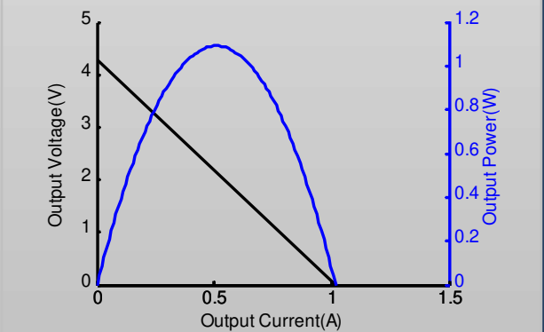
The chart for output voltage and output power Vs output current under Th=150 C and Tc=50 C
